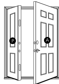
Left/Right Active Swing-Out (L/RASO) shown (R/LASO opposite) (P) Passive and (A) Active
