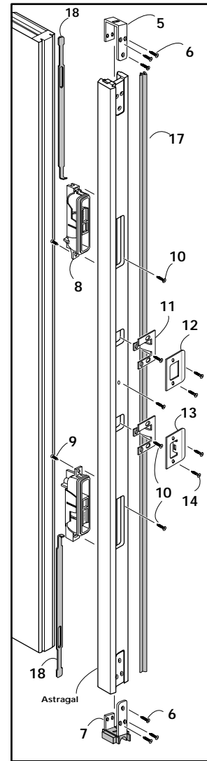
Passive Panel Strike Stile and Astragal
